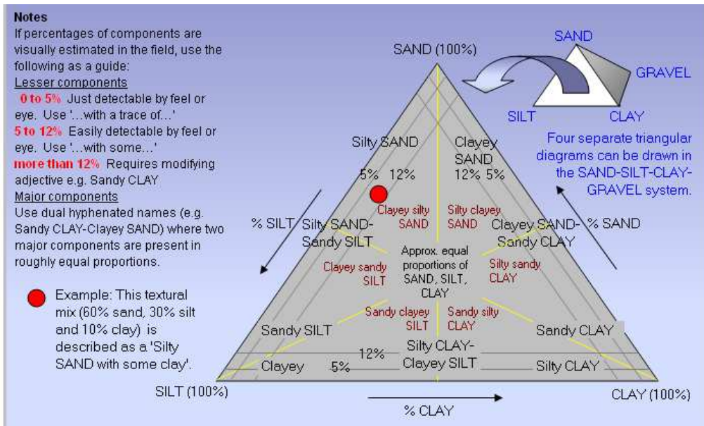
Unified Soil Classification System (USCS; highly recommended)
